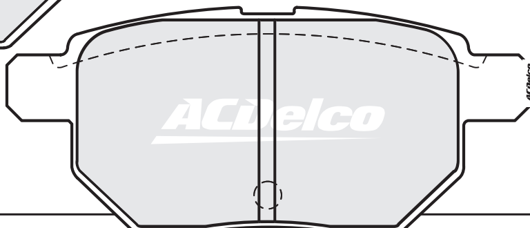
ACD1786 (15.0mm) OUTER TOYOTA
