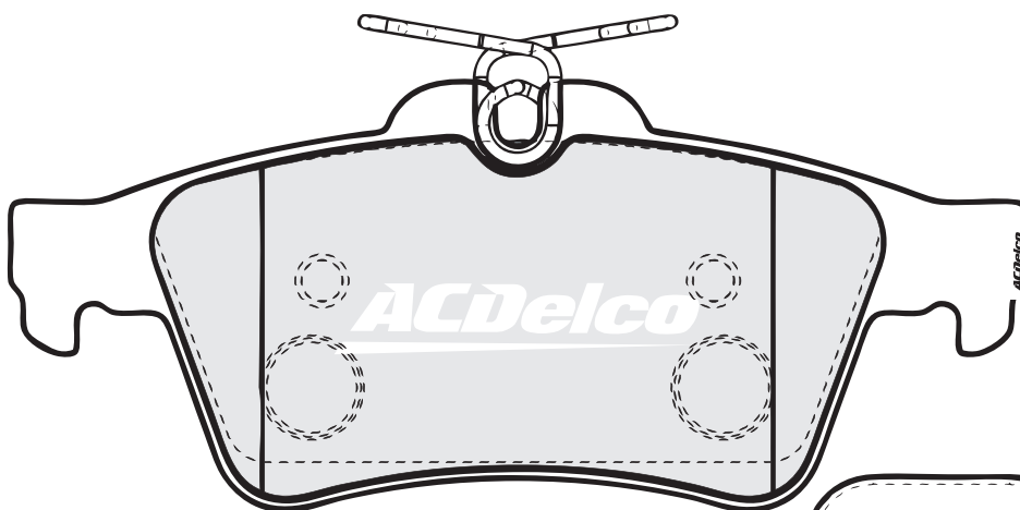
ACD1763 (15.3mm) INNER FORD HOLDEN MAZDA SAAB
