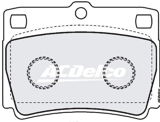
ACD1390 (15.3mm) OUTER
