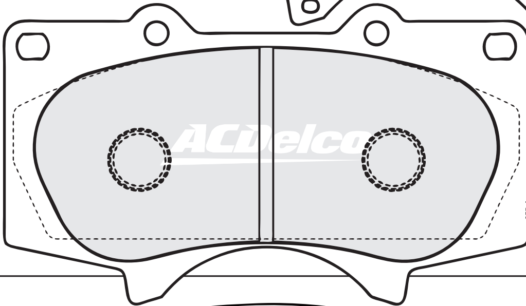
ACD1482 (16.4mm) OUTER MITSUBISHI TOYOTA
