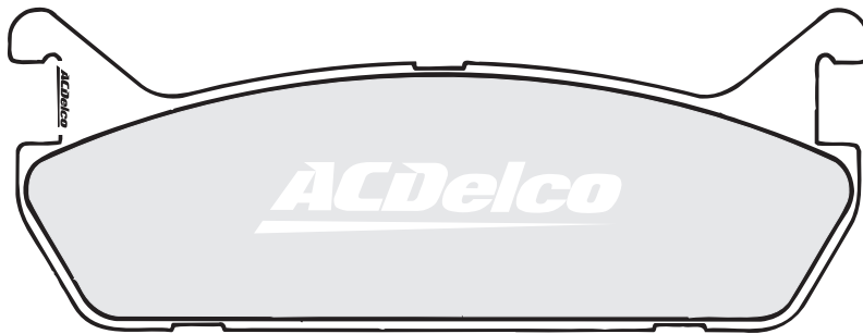
ACD1177 (14.7mm) INNER EUNOS FORD MAZDA
