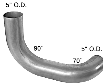
38607 Replaces INTERNATIONAL Part No. 503-845-C1 89" Cab
