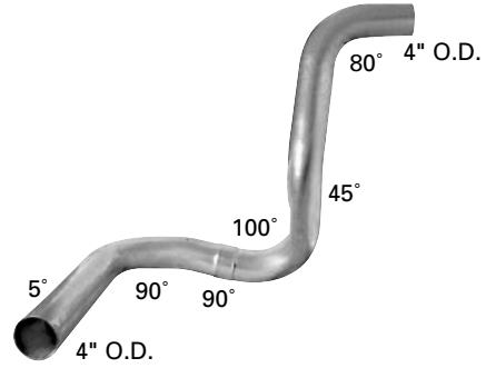
58372 Replaces FORD Part No. E2HZ-5A212F Exhaust Pipe L, LT, LTS 8000 Series with Caterpillar 3208T Engines.
