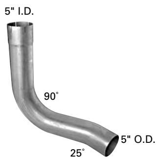
68183 Replaces KENWORTH Part No. 180B-10742-L Left Side Elbow with Offset 868184 - Chrome
