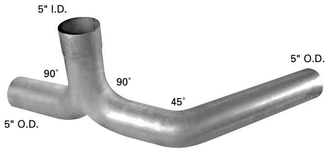
94941 Replaces PETERBILT Part No. 14-04055
