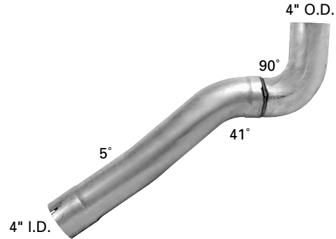
38761 Replaces MACK Part No. 4ME32618 Exhaust Pipe
