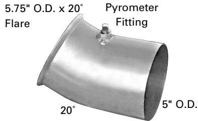
18109 Replaces FORD Part No. D8HZ-5246AC Inlet Pipe RH L, LN, LNT, LT, LTS 9000 Series with Cummins NTC Engines.
