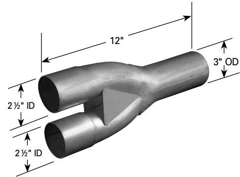
"Y" ADAPTER 92682
