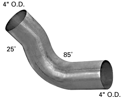
28529 Replaces MACK Part No. 4ME32825 DM Model - Rear Pipe
