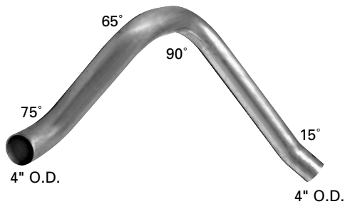
68182 Replaces MACK Part No. 4ME32612 R Model - Round Fuel Tanks
