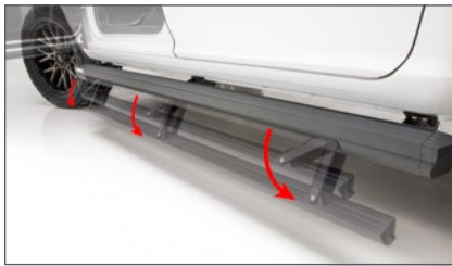
3" powered step automatically drops 8" when door opens, up to 15" below doorsill
