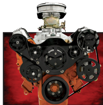
Without AC With Power Steering #BLK13805
