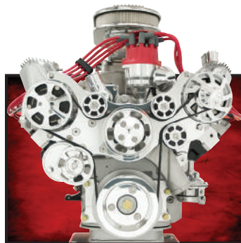
With AC Without Power Steering #14720
