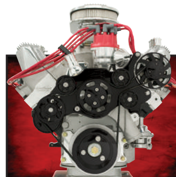
Without AC Without Power Steering #BLK14725
