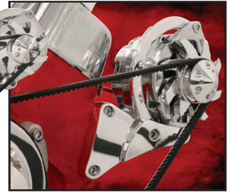
BIG BLOCK CHEVROLET® - STANDARD HEADS Independent Side Mount- Alternator Bracket
