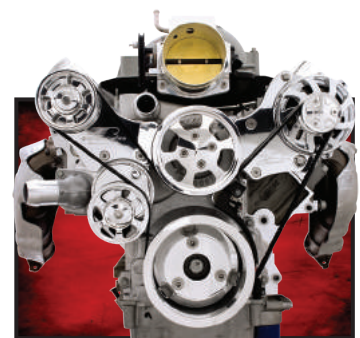
Without AC Without Power Steering #13475
