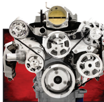
Without AC With Power Steering
