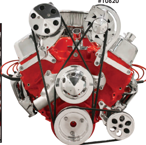
BIG BLOCK CHEVROLET® - STANDARD HEADS Independent Top Mount- Alternator Bracket
