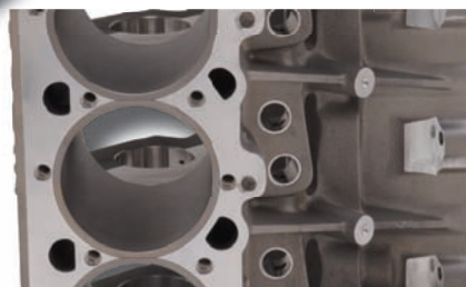
SLEEVES WITH THICK REGISTERS INSTALLED ASSURING PROPER RING SEAL
