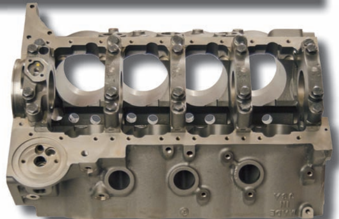
PRIORITY MAIN OILING
