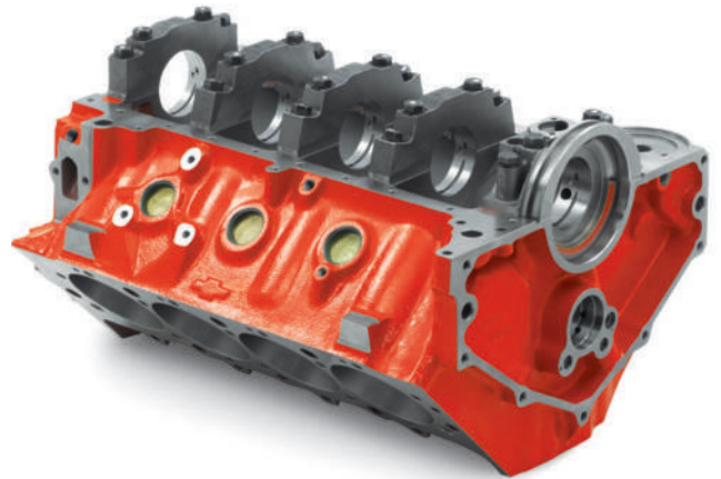
A Tall Deck Bowtie Sportsman Bare Block (bottom, rear)
