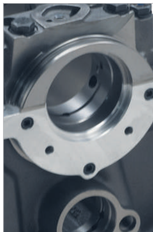
2-Piece Rear Main Seal C
