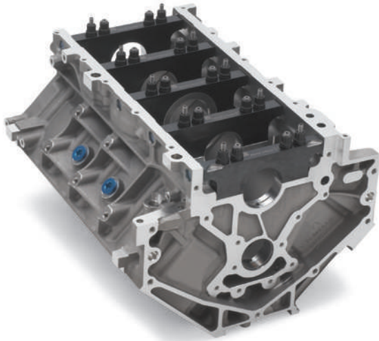
Aluminum C5R Racing Block (bottom, rear) B
