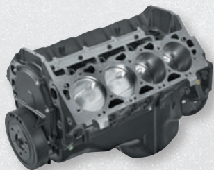
12568782 502 Partial Engine This brand-new Partial engine includes forged reciprocating components, as well as the balancer, oil pan and timing chain set.
