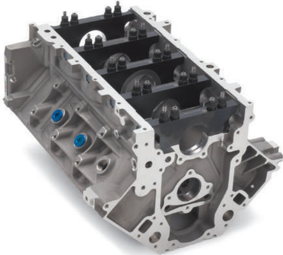
Aluminum C5R Racing Block (bottom, front) B
