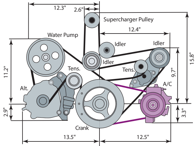
B LT4 Wet Sump (ZL1 Camaro) Accessory Drive System (19332590) with LT4 Wet Sump & LT1 Camaro A/C Add-on Kit (19332591)
