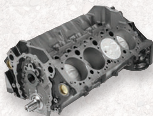
12670966 SP/ZZ Partial Engine The SP350 Partial is based on the popular ZZ4 partial engine assembly and includes the forged steel crankshaft, high-silicon pistons and connecting rods.
