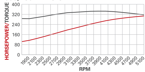
DYN0 CHART
