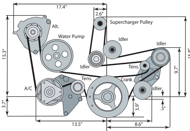
LT4 Dry Sump Accessory Drive System, with A/C D
