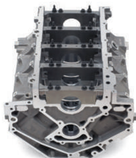
LS3/L92 Aluminum 6.2L Bare Block (bottom, front) B
