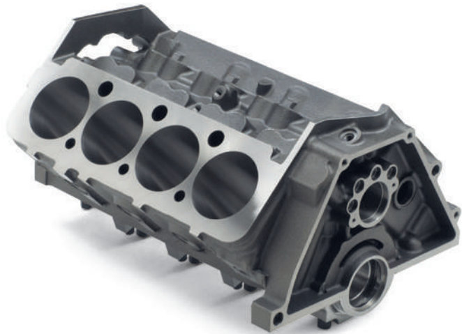
A Short-Deck Race Block (top, rear)
