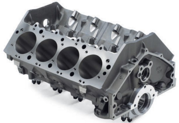
A Tall Deck Bowtie Race Bare Block (top, rear)
