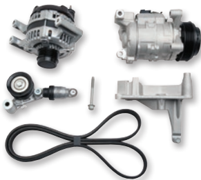
12679459 LT1 Accessory Drive System Page 285
