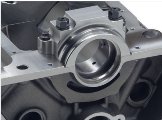
2-Piece Rear Main Seal A
