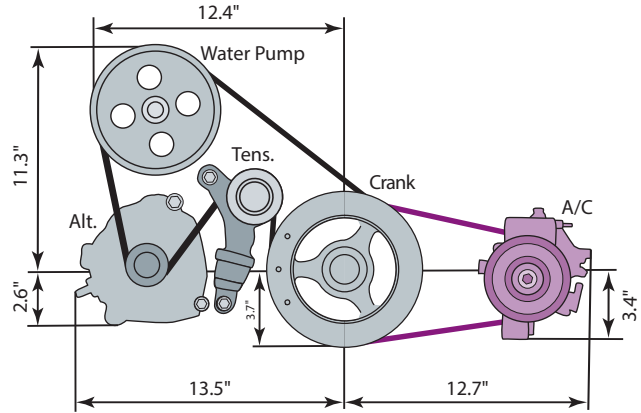
A LT1 Camaro Wet Sump Accessory Drive System (12678595) with LT4 Wet Sump & LT1 Camaro A/C Add-on Kit (19332591)
