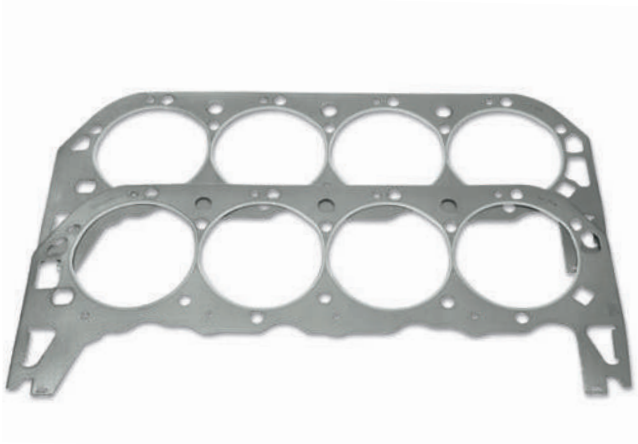
B Head Gasket Kit, 502 Engine
