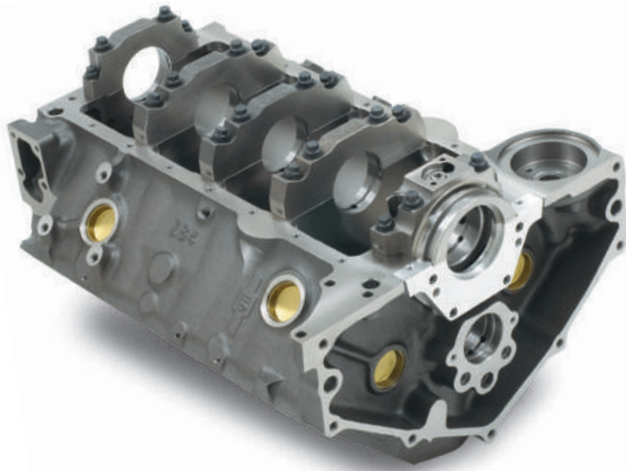
350 Bowtie Sportsman Block, 2-Piece Rear Main Seal B
