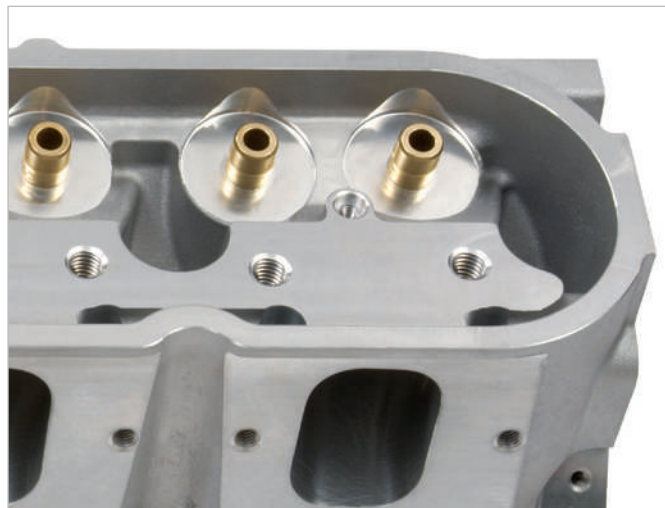
D LSX-DR Rocker Stand Pads
