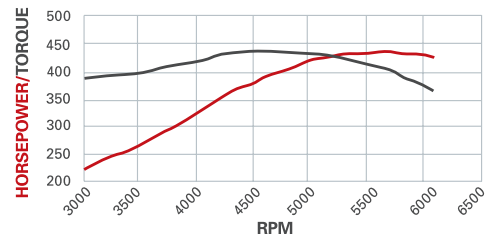
DYN0 CHART
