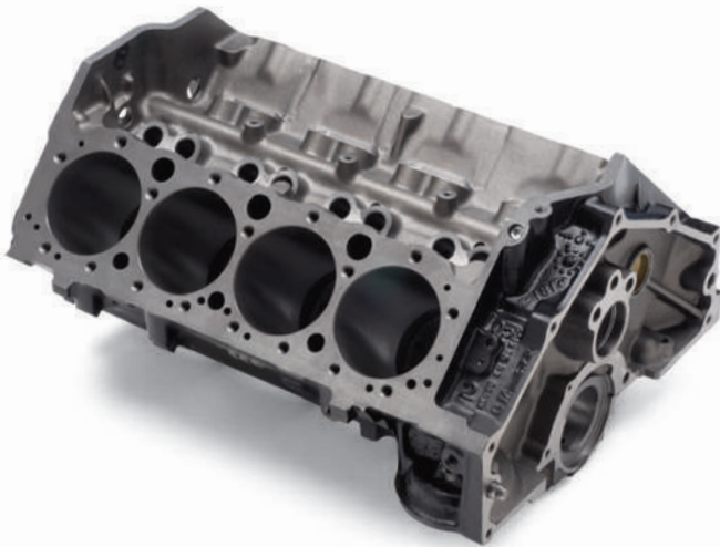
Production-Based Block (top, rear) A
