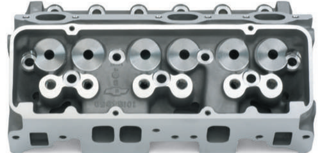
A 18° Aluminum Cylinder Head (top/intake)
