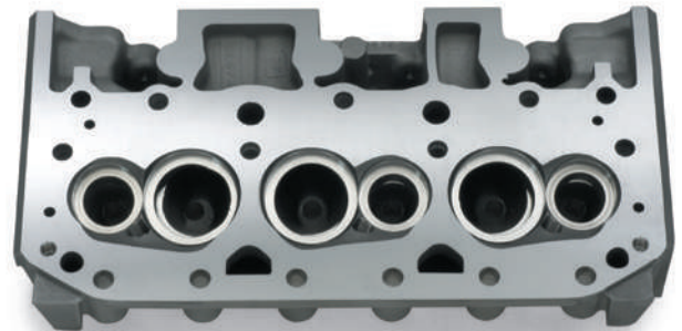
A 18° Aluminum Cylinder Head (combustion chamber)
