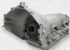
19300175 SuperMatic™ 4L85-E Four-Speed Automatic Transmission Features five-pinion gearsets, heat-treated stator shaft splines, induction-hardened turbine shaft, seven-plate clutch and specific valve-body calibration. See page 366 for torque converter applications.
