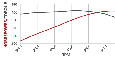
DYN0 CHART
