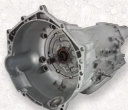
19368611 SuperMatic™ 4L65-E Four-Speed Automatic Transmission (remanufactured) Electronically controlled four-speed overdrive transmission. Suitable for engines producing up to 430 lb.-ft. of torque.
