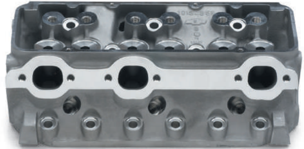
A 18° Aluminum Cylinder Head (exhaust)
