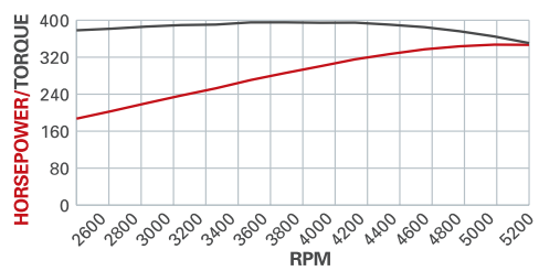
DYN0 CHART
