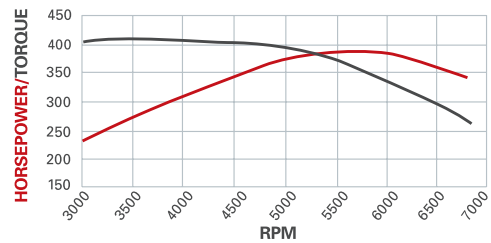
DYN0 CHART
