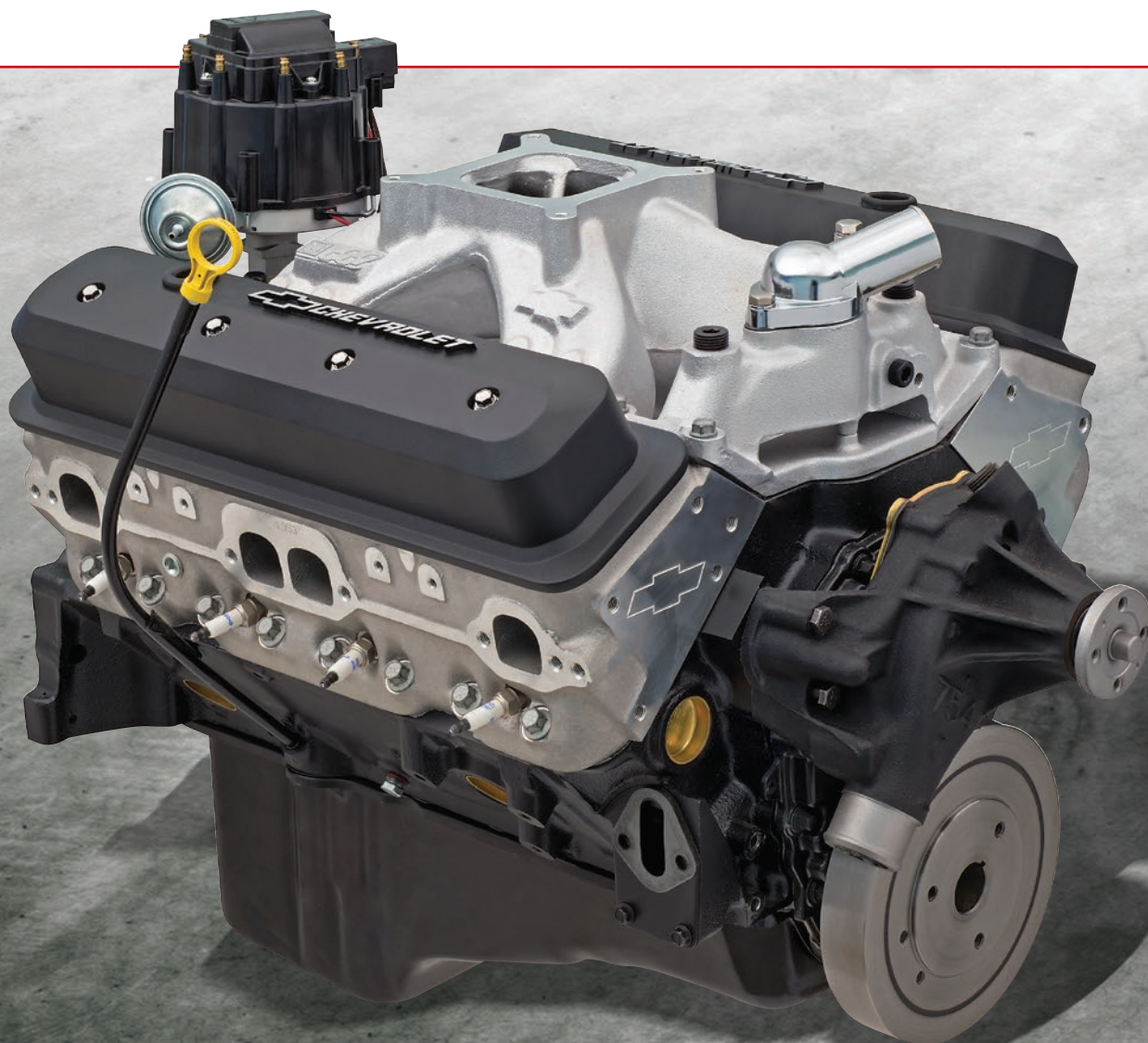
12670966 SP/ZZ Partial Engine The ZZ6 is based on the popular ZZ4 partial engine assembly and includes the forged steel crankshaft, high-silicon pistons and connecting rods.
