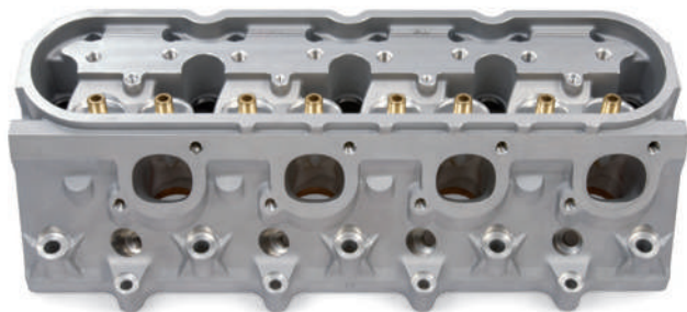
LSX-CT CNC-Ported Cylinder Head (exhaust) B
