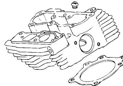
Cometic Part #-C9153 Valve Stem Seal Hat Style Viton 2003-Present Replaces: 18094-02
