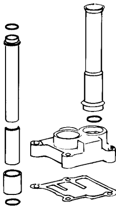
Cometic Part #-C9578 Lifter Cover 1999-UP Replaces: 18635-99
