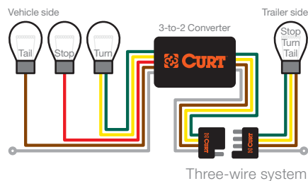
Three-wire system
