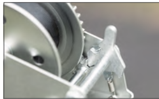
Broached pinion shaft securely engages the pinion gear
