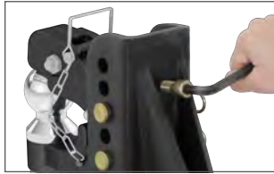
Built-in anti-rattle helps promote quiet towing (select models)
