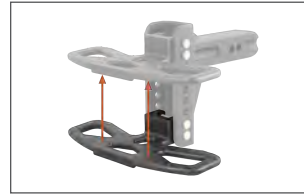
Channel attachment allows for versatile height adjustment
