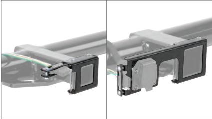
Slotted holes to fit multiple connector types (varies by part number, see table below)
