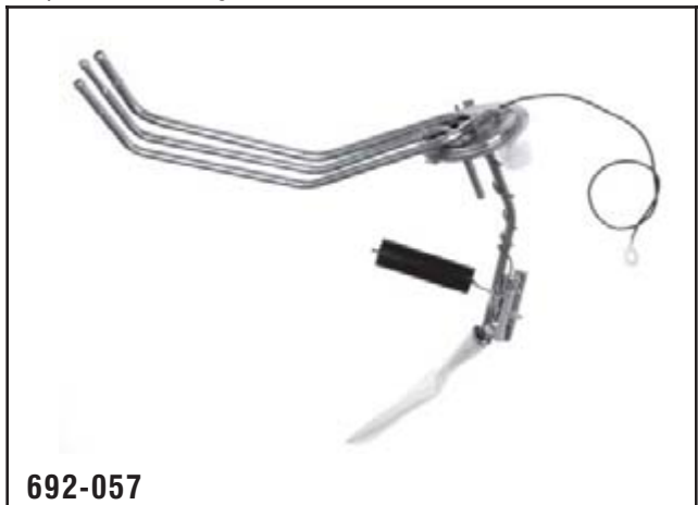
692-057 GM (Inc. Truck) Number of Outlets: 3 1990-77 Bonneville, Caprice, Catalina, Custom Cruiser, Estate Wagon, Safari Full size RWD, w/E.E.C., w/o FI S.W. only.
