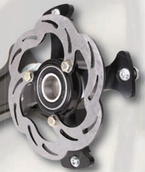
#25605 Micro Sprint Front Hub w/ Brake Rotor Flange shown.
