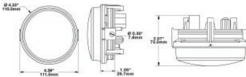
FIXED MOUNT
