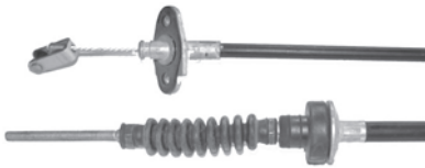
CA-676 Description: Clutch Overall Length: 22.75 Mounting Length: 15.25
