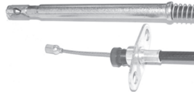
Part no.: CA-8432 Description: Accelerator Cable Overall Length: 32.08 Mounting Length: 19.88
