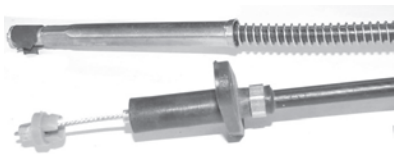
Part no.: CA-8453 Description: Accelerator Cable Overall Length: 19.96 Mounting Length: 9.468
