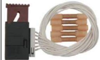
S1048 Accelerator Pedal Sensor Connector 89046653
