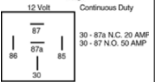
RY30 A/C Auto Temperature Control Relay
