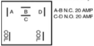
RY32 A/C Compressor Clutch Cut-Off Relay
