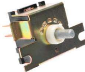
HS242 A/C and Heater Blower Motor Switch 16068778; 16068777; 16015450
