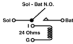
SR113 Starter Relay J3236793; 3236793; 5758600; 12323110
