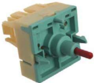
HS386 A/C and Heater Selector Switch 2L1Z-19B888-AA Ford ..... 2006 - 2003
