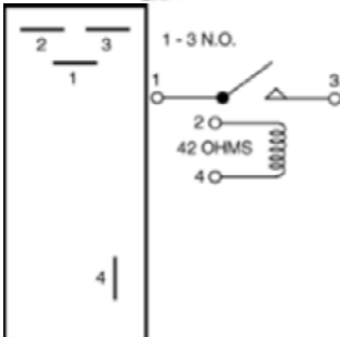
RY74 A/C Compressor Clutch Cut-Off Relay 4339495; 4221576; 4221272; 88922580
