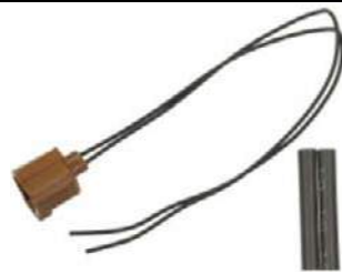
S1082 Coolant Temp Sensor Connector 3U2Z-14S411-LXA
