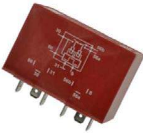
RY1791 Multi-Function Relay 9566647; 4433801
