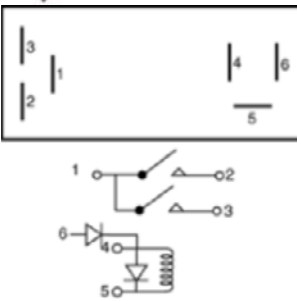
RY79 Auxiliary Engine Cooling Fan Relay 4221615; 5227415; 5226915; 4419169
