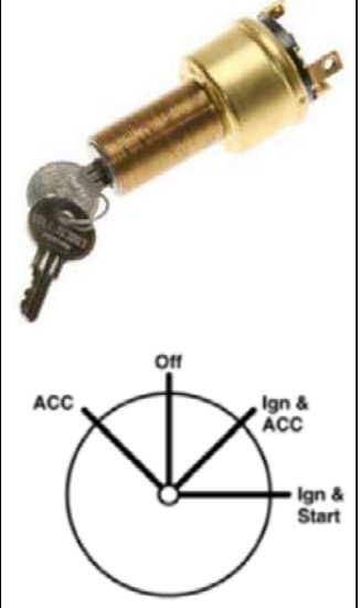
US129 Ignition Starter Switch
