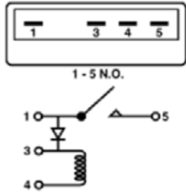
RY76 A/C Comp Throttle Cut-Off Relay 14048054
