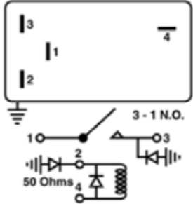
RY72 Auxiliary Engine Cooling Fan Relay 4221542; 4221661; 4221684; 4221287
