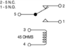
RY31 A/C Compressor Clutch Relay
