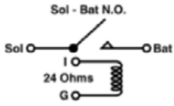
SR109 Starter Relay 2875618
