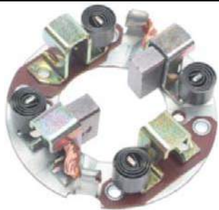
JX140 Starter Brush Set 28140-26070
