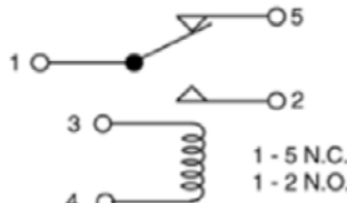
RY23 Air Control Valve Relay 89057581; 463468
