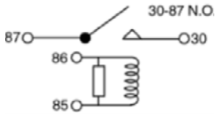
RY255 A/C Relay
