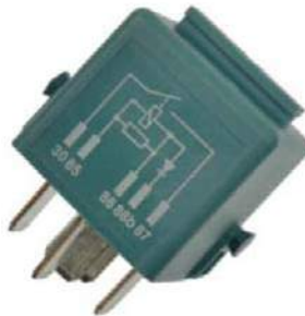
RY1796 Multi-Function Relay 61361388910; 61311388912; 61311378797
