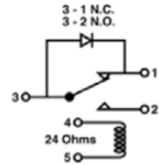
SR115 Starter Relay 4145370; 12309860
