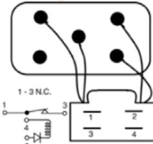
RY957 Fuel Shut-Off Relay Honda..... 1975 - 1974
