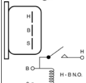
HR114 Horn Relay
