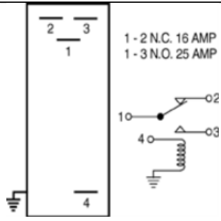
RY-8 A/C Auto Temperature Control Relay
