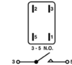
RY-601 A/C and Heater Relay 8191150800; 8191160570; 8153934120; 13500114; 8120885670; 8121936110; 19115083; 19115080; 13502679; 12135170; 12088567
