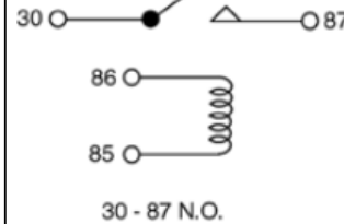
RY-193 A/C Compressor Clutch Cut-Off Relay 4504206; 5233205; 4443907
