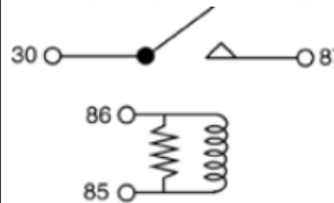
30 - 87 N.O. RY-531 A/C Control Relay 12077867
