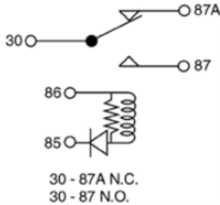
RY-145 A/C and Heater Relay 25526984; 22526984; 12395259; 4373109
