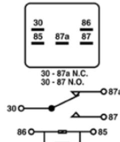
RY-604 A/C Condenser Fan Motor Relay 8192590190; 8153288650; 8135031030; 8121936120; 8121936050; 8121936020; 8121772340; 8121351980; 8219974080; 12077865; 96263403; 19116363; 19115298; 3886078J01; 21997408; 15328865; 12193612; 12177234; 12193602; 12135198
