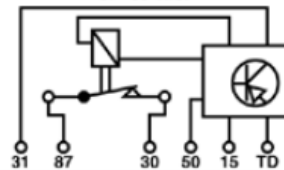
RY-191 Accessory Relay 0015450605; 15450605; 00015450705; 00015450605
