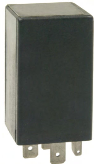
RY-1340 A/C Compressor Clutch Cut-Off Relay 1H0919577; 1H0919577
