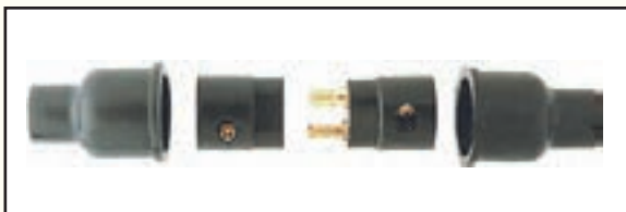
TC20 (Set) 2-Pole Trailer Connector • Hard rubber body, soft rubber end caps • All brass, metal components, polarized • Accepts up to 12 ga. wire
