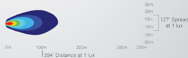
CTL-EPX1140 | 9112367 - 40° BEAM
