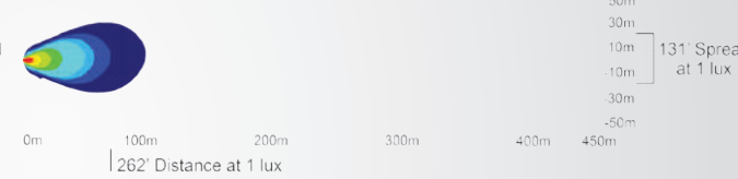
MIL-RXP1060T | 4009998 - 60° Beam
