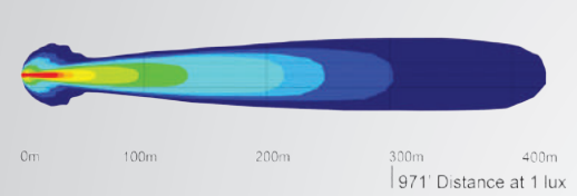
MIL-RXP1210T | 4009974 - 10° Beam
