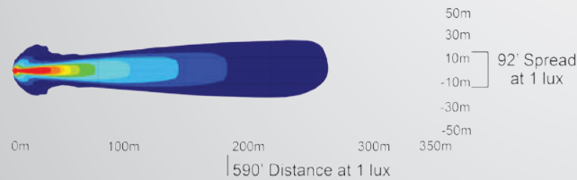
CTL-EPX1110 | 9112183 - 10° BEAM
