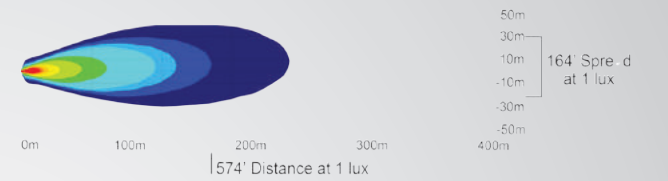
CTL-TPX1840 | 9119748 - 40° BEAM
