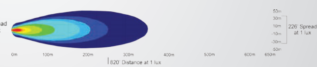
XIL-PX2-1840 | 9116235 - 40° BEAM
