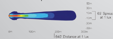
XIL-LPX910 | 4000773 - 10° BEAM
