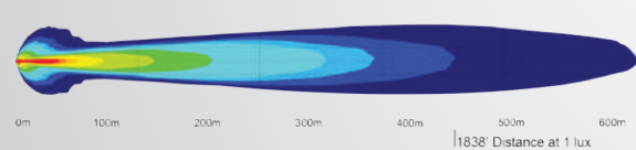
XIL-PX2.1810 | 9116143 - 10° BEAM
