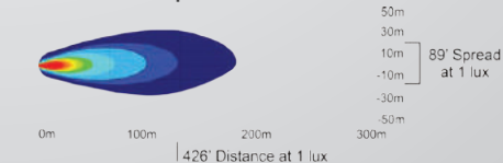
XIL-LPX940 | 4000780 - 40° BEAM
