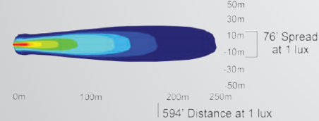
XIL-SP520 | 4009844 - 20° Beam
