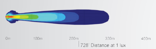
MIL-RXP1210T | 4009974 - 10° Beam
