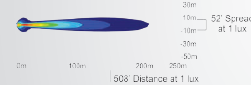
XIL-UMX4410 | 4004726 - 10° BEAM
