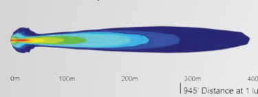
XIL-PX1810 | 9115788 - 10° BEAM
