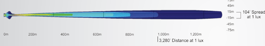
CTL-CPZ810 | 9890852 - 10° BEAM
