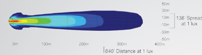
CTL-TPX1810 | 9111018 - 10° BEAM
