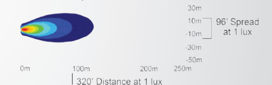
XIL-UMX4440 | 9118390 - 40° BEAM
