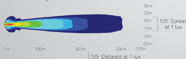
CTL-EPX1110 | 9112183 - 10° BEAM
