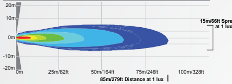
XIL-SP110 | 4008830 - 10° BEAM
