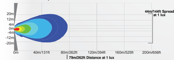
MAR-RXP1260 | 9892092 - 60° Beam
