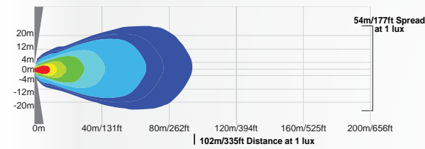
MAR-RXP2060 | 9892108 - 60° Beam
