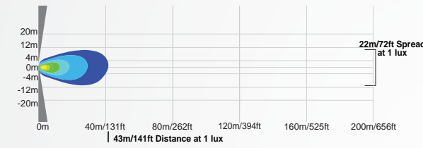
MAR-EPX760 | 9892115 - 60° Beam
