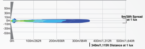
CTL-CPZ110XP | 9893259 - 10° BEAM
