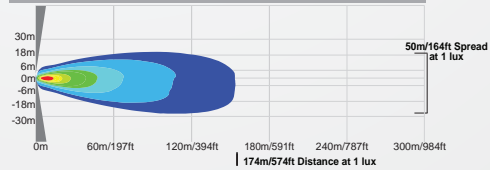
CTL-TPX1840 | 9111193 - 40° BEAM
