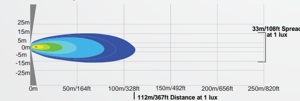
BHB070540 | 9897998 - 40° Beam
