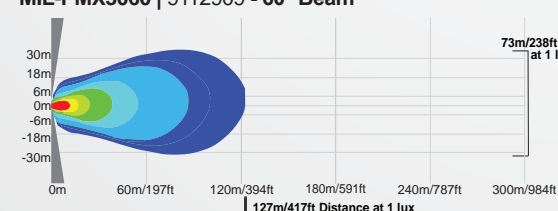
MIL-PMX3060 | 9112909 - 60° Beam
