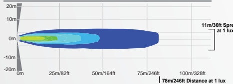
XIL-S1110 | 9888156 - 10° BEAM
