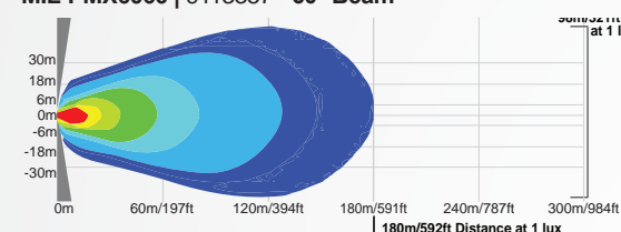
MIL-PMX6060 | 9113357 - 60° Beam
