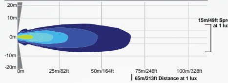
XIL-SP120 | 4009882 - 20° BEAM
