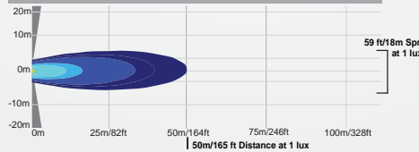
XIL-MX140 | 9113715 - 40° BEAM
