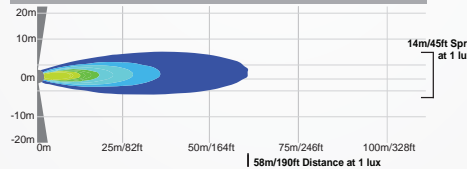
XIL-S1130 | 9888163 - 30° BEAM
