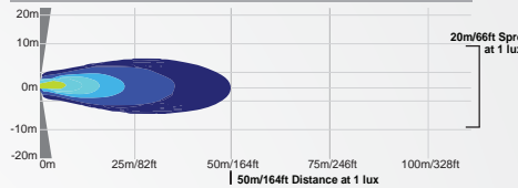
XIL-SP140 | 4009899 - 40° BEAM
