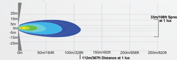
BLB070540 | 9897998 - 40° Beam
