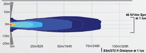
XIL-MX110 | 9113531 - 10° BEAM
