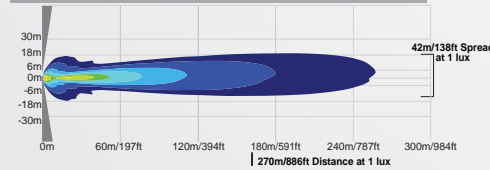
CTL-TPX1810 | 9111018 - 10° BEAM
