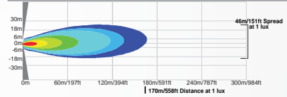
XIL-PX1840 | 9115870 - 40° BEAM
