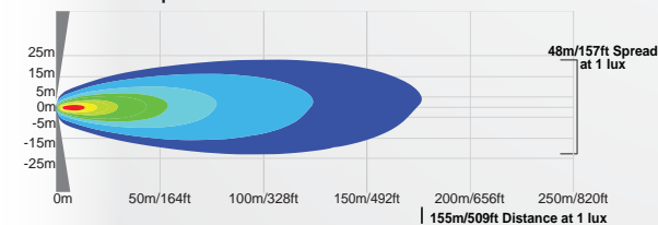
BLB071240L | 9898117 - 40° Beam
