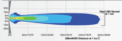
XIL-PX1810 | 9115788 - 10° BEAM
