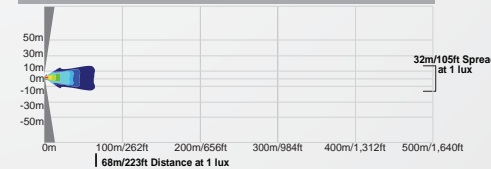
XIL-OP260 | 9139548 - 60° BEAM
