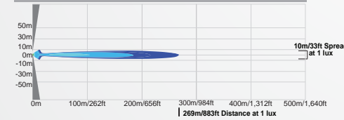
XIL-OP110 | 9123882 - 10° BEAM
