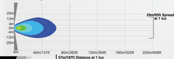
DURA-M460 | 9895499 - 60° Beam
