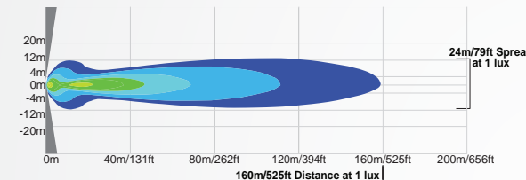
DURA-610 | 9891125 - 10° Beam
