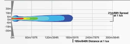
XIL-LPX910 | 4000773 - 10° BEAM
