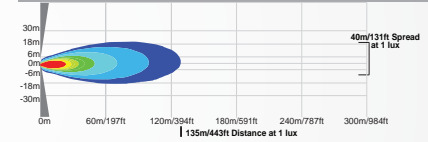
XIL-LPX940 | 4000780 - 40° BEAM
