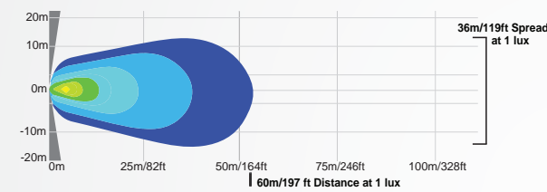
XIL-UMX4060 | 9118307 - 60° Beam
