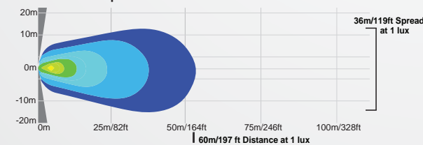
XIL-UMX4460 | 9118482 - 60° Beam
