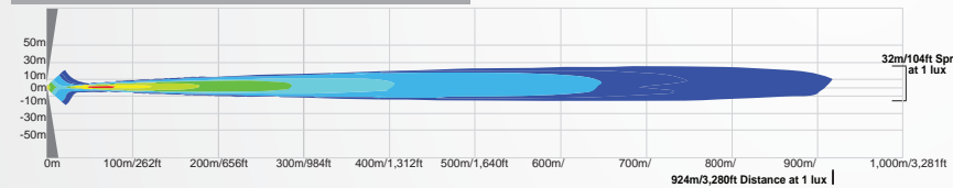
CTL-CPZ810 | 9890852 - 10° BEAM
