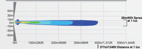
XIL-OP210 | 9124605 - 10° BEAM
