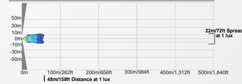
XIL-OP160 | 9124063 - 60° BEAM
