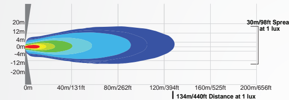
XIL-SP740 | 4009875 - 40° Beam
