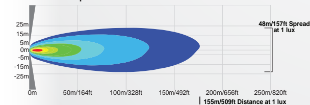
BHB071240L | 9898179 - 40° Beam
