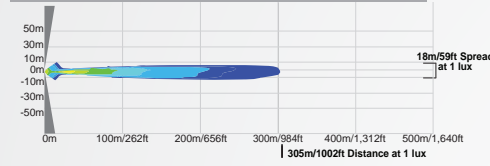
CTL-CPZ110 | 9150970 - 10° BEAM
