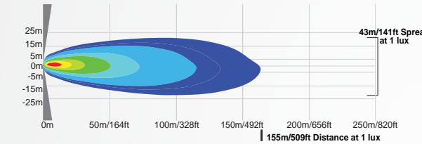
BLB070940 | 9898056 - 40° Beam
