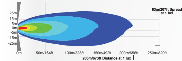
BHB072040 | 9898230 - 40° Beam
