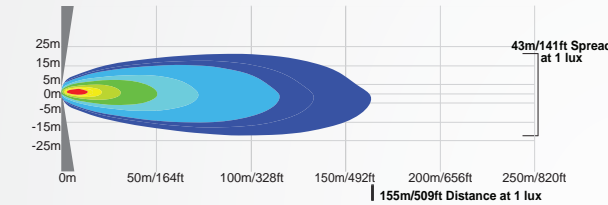
BHB070940 | 9898056 - 40° Beam
