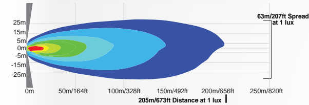
BLB072040 | 9898230 - 40° Beam
